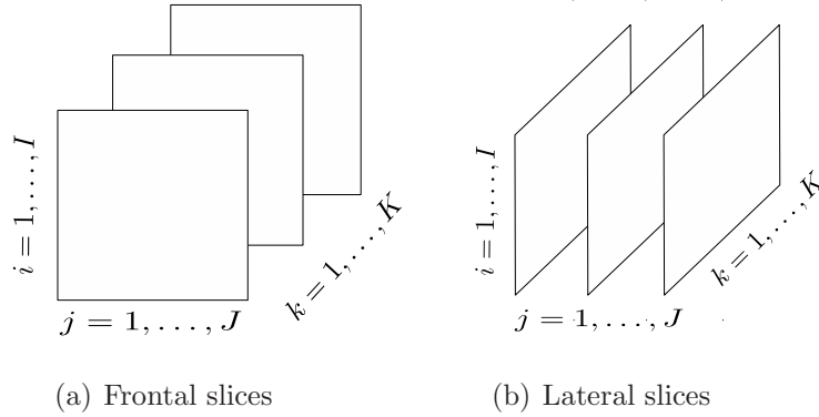
Figure 1: Frontal ( \mathbf{P}_{..k} ) and lateral ( \mathbf{P}_{.j} ) slices of the tensor \underline{\mathbf{X}} that are handled within MGCCA
